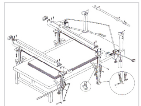
Installation Diagram
