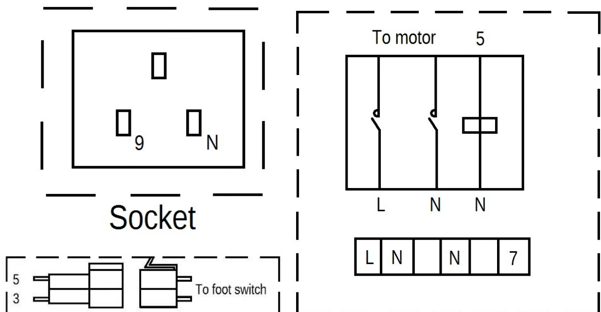
Figure 4 : Electrical Schematic Diagram of KW-303 Ironing Table
