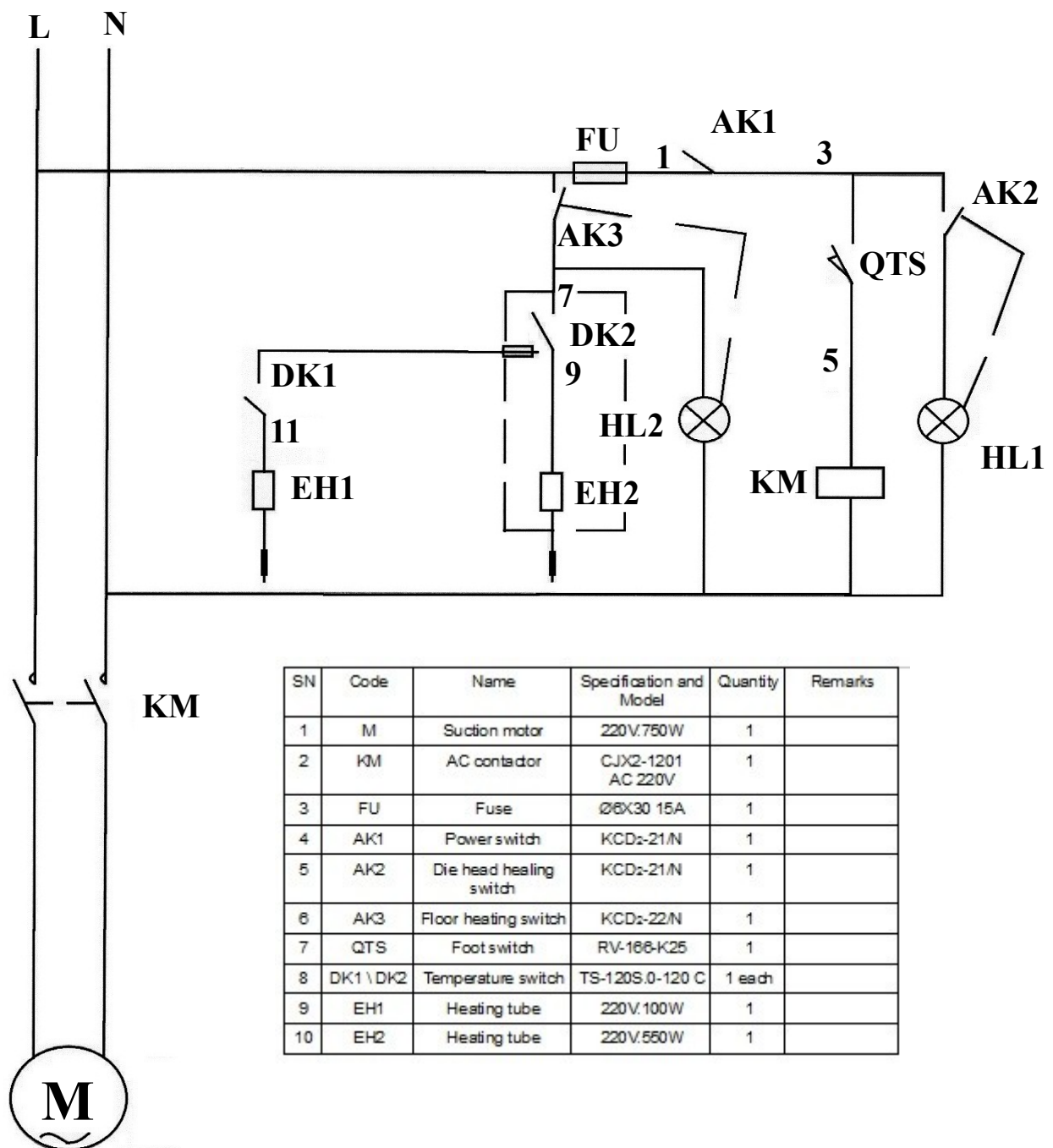
Figure 4 : Electrical Schematic Diagram of KW-303 Ironing Table
